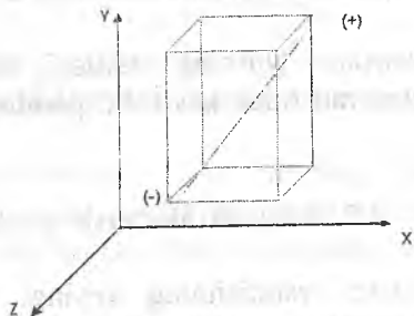
2.20-rasm. Parallelepiped.
