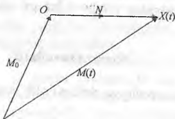
2.19-rasm. Nur.
