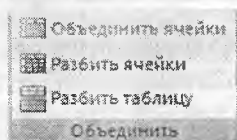
9.11-rasm. Birlashtirish.
