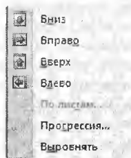
9.32-rasm. Progressiya.
