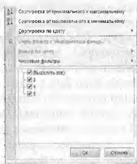
9.40-rasm. Saralash.
