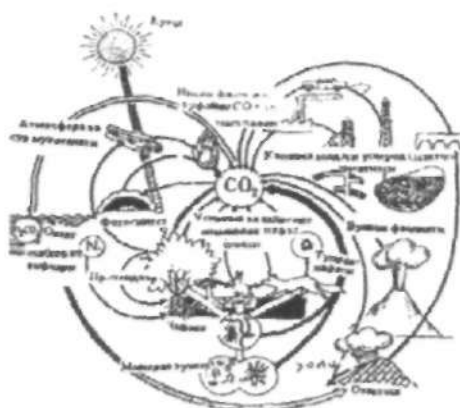
18-rasm. Uglerodning biosferada aylanishi.
