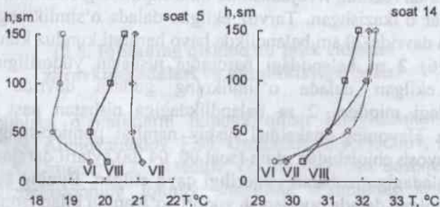
12.5-rasm. Sholi dalasida iyun-avgust oylarida soat 5 (a) va 14 (b) da havo haroratining vertikal taqsimlanishi (1997–1999-yillar)
