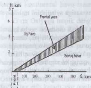
10.2-rasm. Frontal yuza va front chizmasi
