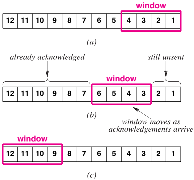
Figure 26.2 An illustration of a sliding window in (a) initial, (b) intermediate, and (c) final positions.
