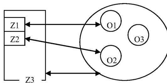
Figure 8: A Partition with Empty Space.
