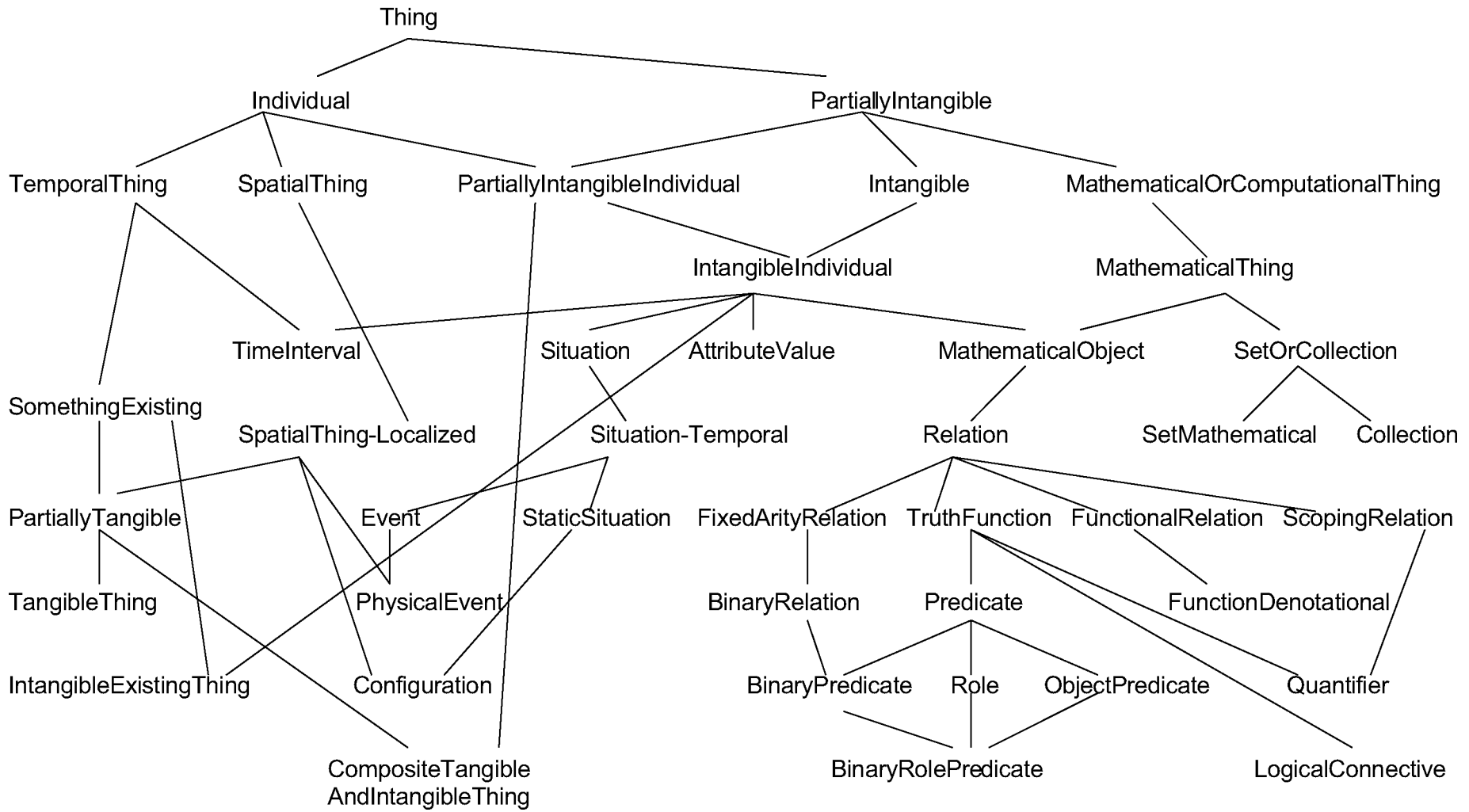
Figure 2: The OpenCYC Upper Ontology. Source: http://www.cyc.com/cyccdoc/upperont-diagram.html
