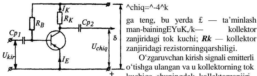
22.16- rasm. \delta dagi rezistorning kuchlanish tushishiga
