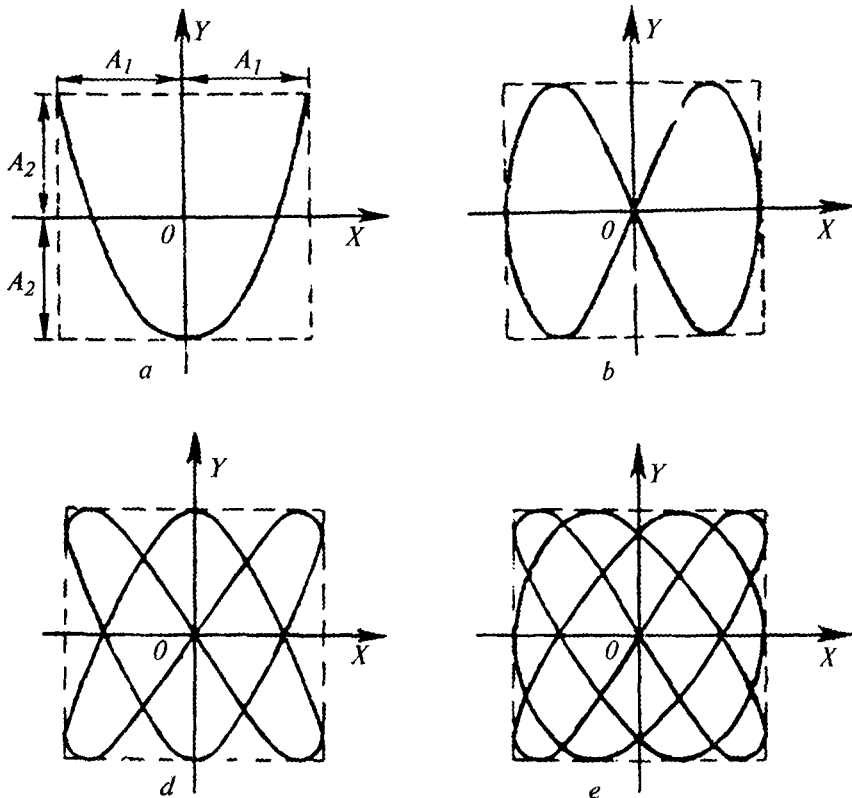
7.13- rasm. a) ( \omega_1/\omega_2=1/2 , \Phi_{01}\sim\Phi_{02}=0 ;
