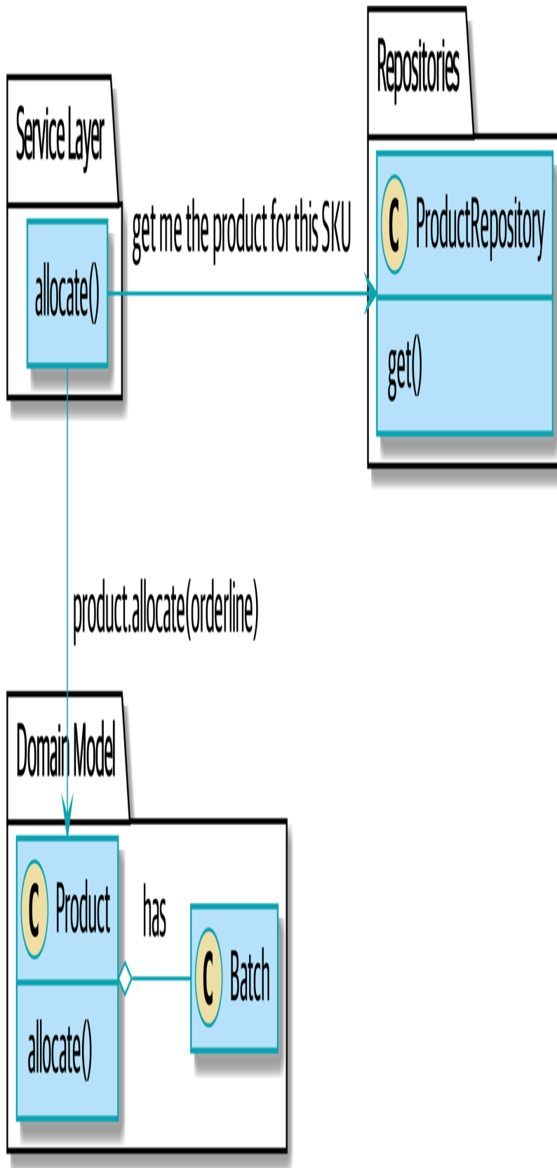
Figure 7-3. After: ask Product to allocate against its batches
