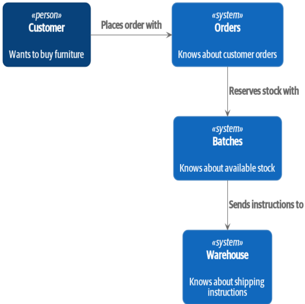
Figure 11-2. Context diagram with noun-based services
