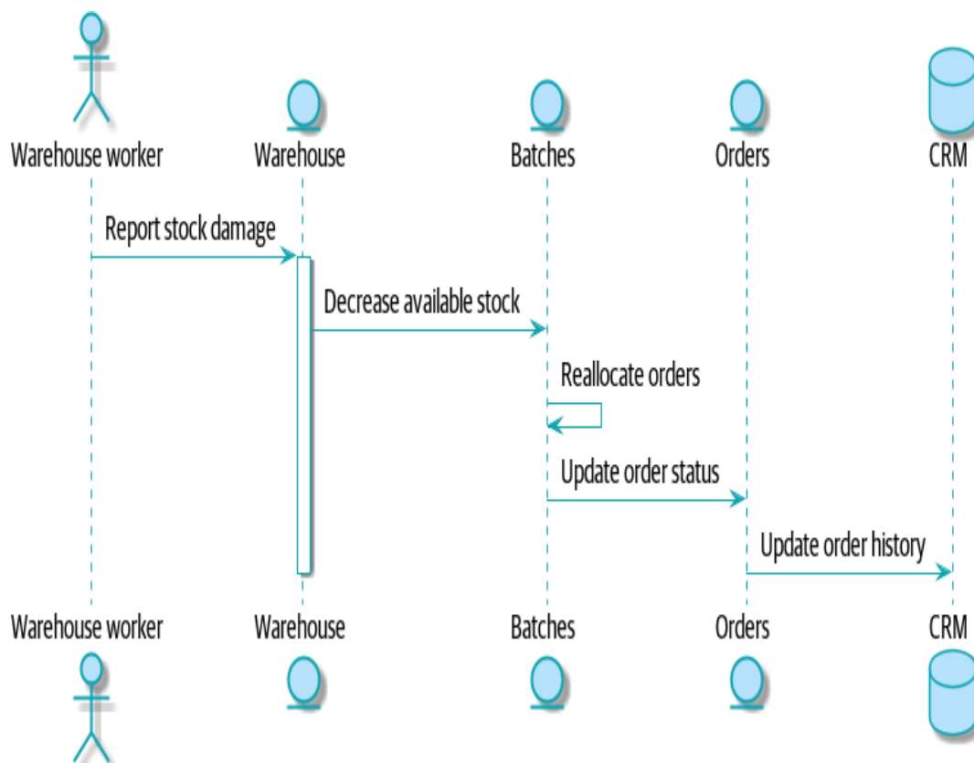
Figure 11-4. Command flow 2
