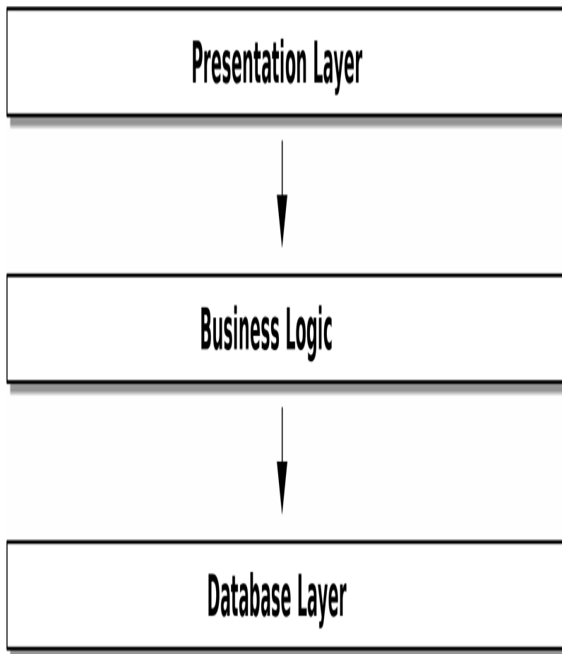
Figure 2-2. Layered architecture
