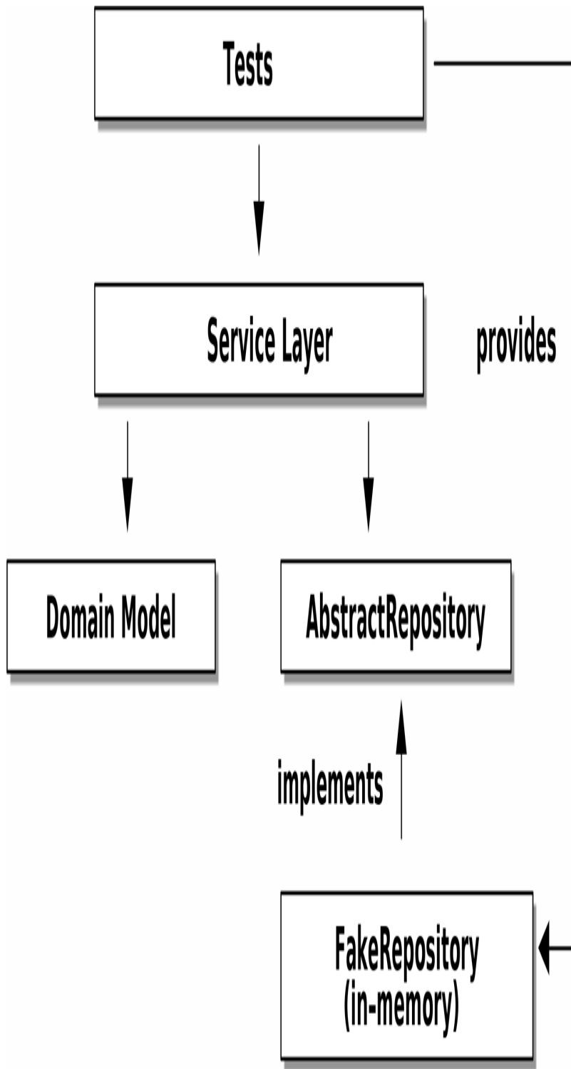
Figure 4-4. Tests provide an implementation of the abstract dependency
