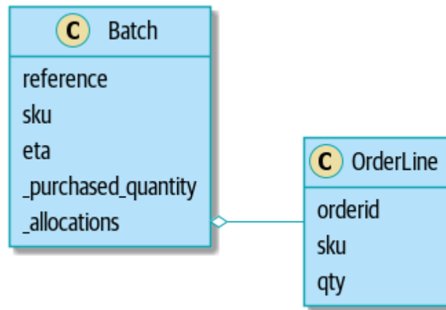
Figure 2-4. Our model
