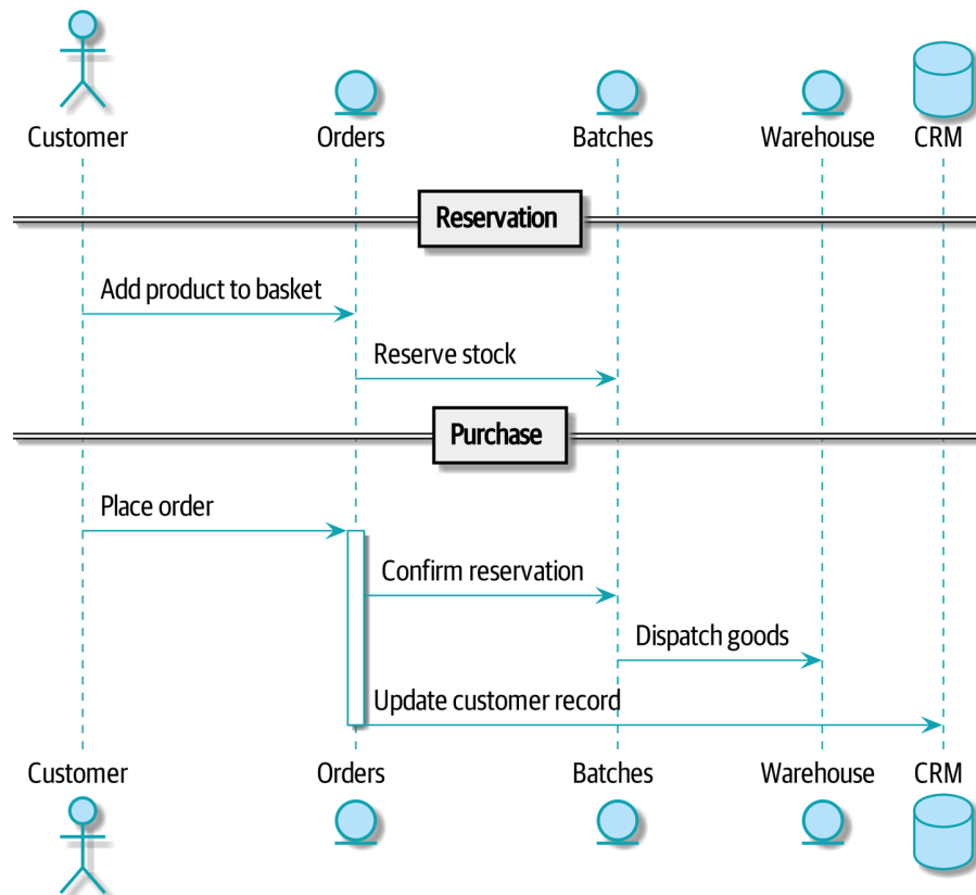
Figure 11-3. Command flow 1
