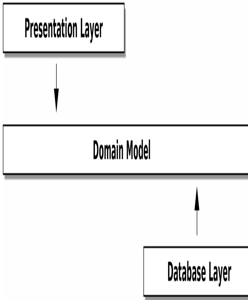
Figure 2-3. Onion architecture
