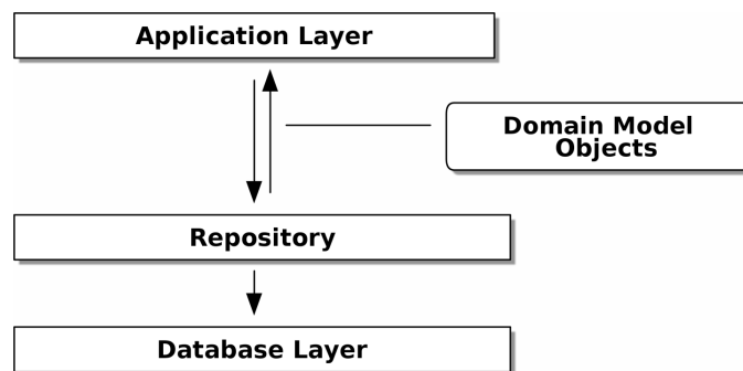
Figure 2-5. Repository pattern
