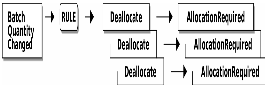
Figure 9-3. Batch quantity changed means deallocate and reallocate
