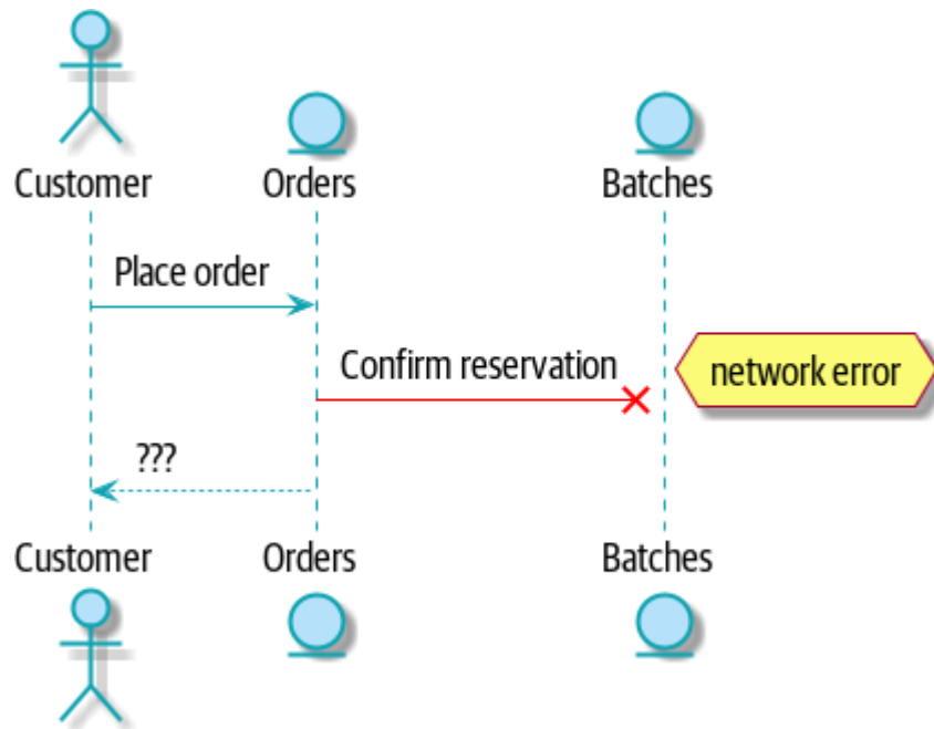
Figure 11-5. Command flow with error
