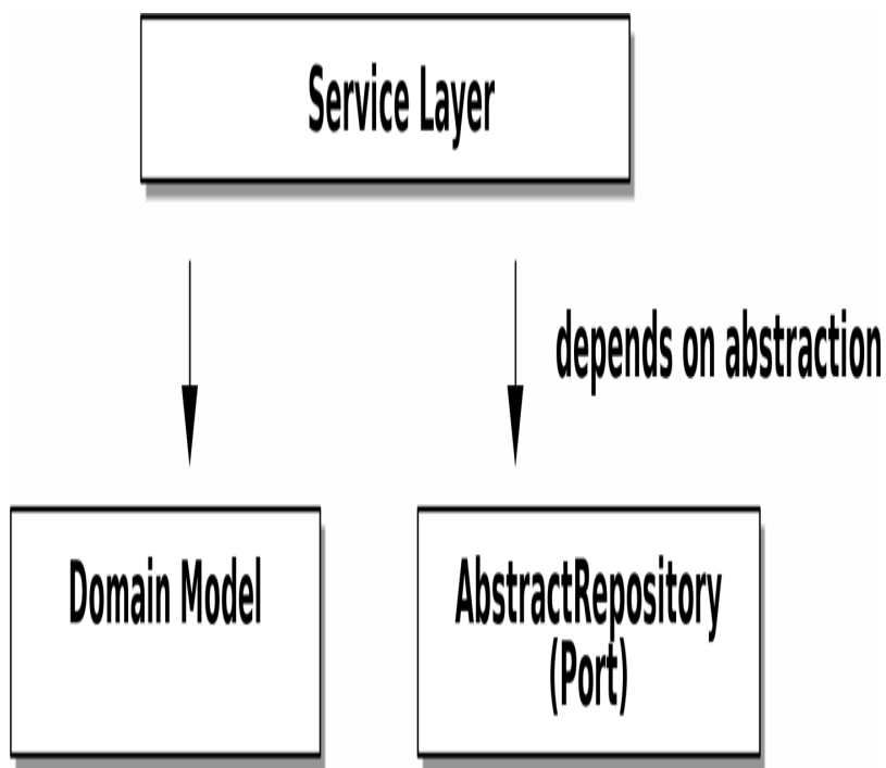
Figure 4-3. Abstract dependencies of the service layer
