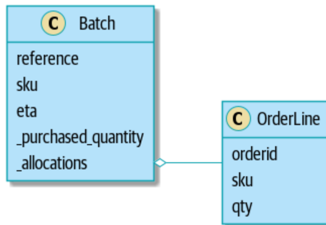
Figure 1-3. Our model in UML
