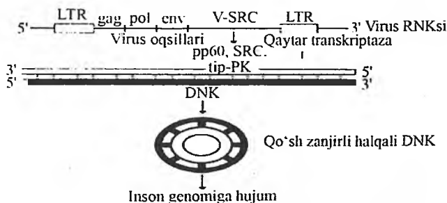
7.5-rasm. Raus virusi genomining tuzilishi
